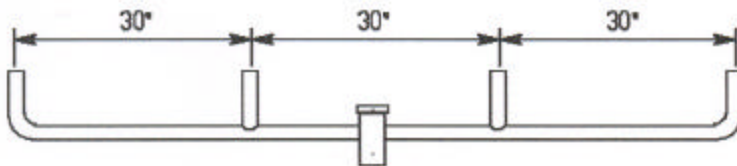
TYPE 'H' BULLHORN
